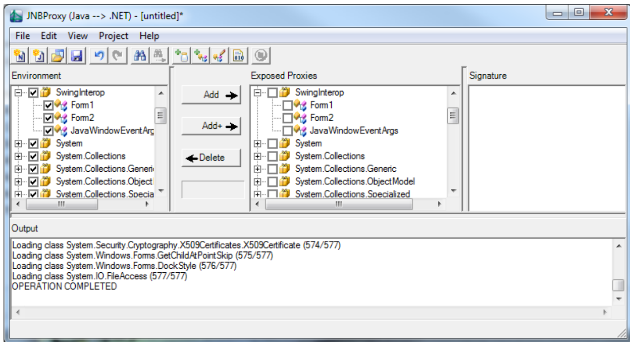
Figure 8. After adding classes to Exposed Proxies pane
