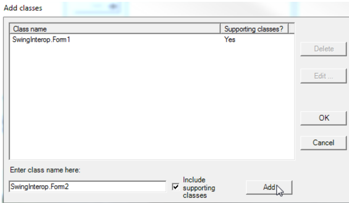
Figure 6. Adding a class from the classpath
