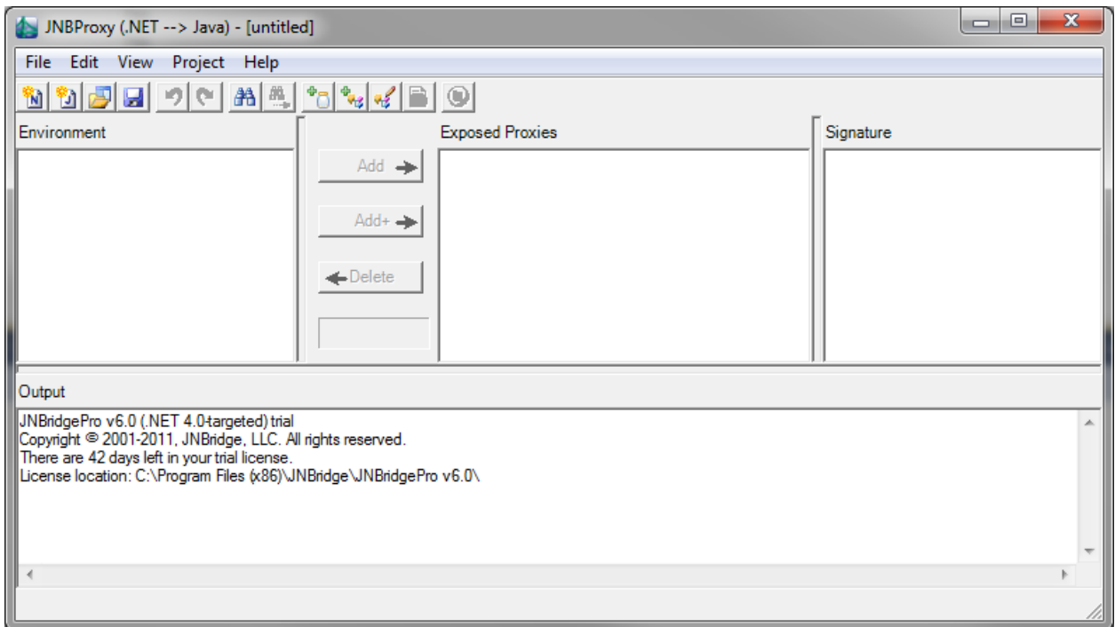
Figure 2. JNBProxy
